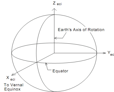
Figure 4. Earth Centered Inertial (ECI) Coordinate System
